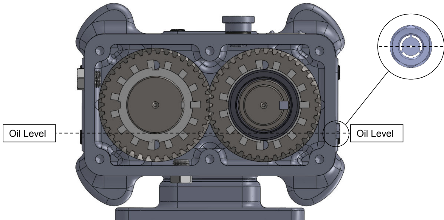
Frame 5 Only - Sight glass located in the lowermost position on the side of the gearbox
